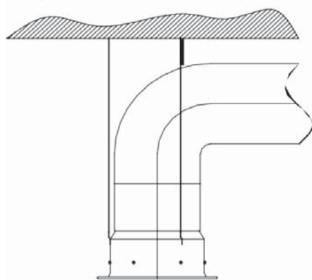
FIG. 3 INSTALLATION ON FLEXIBLE HOSE
