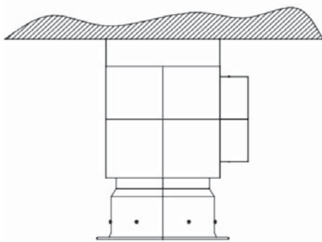
FIG. 4 INSTALLATION WITH PLENUM
