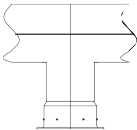
FIG. 2 INSTALLATION ON DUCT WITH CONNECTING SLEEVE
